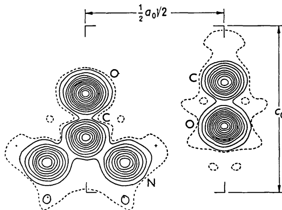
Fig. 2. Electron-density section \rho(x, \frac{1}{2} + x, z) . Solid contour lines are drawn at 1, 2, 3, ... e \cdot \text{Å}^{-3} ; the broken contour line is at \frac{1}{2} e \cdot \text{Å}^{-3} . The small crosses indicate the positions assigned to the hydrogen atoms.
